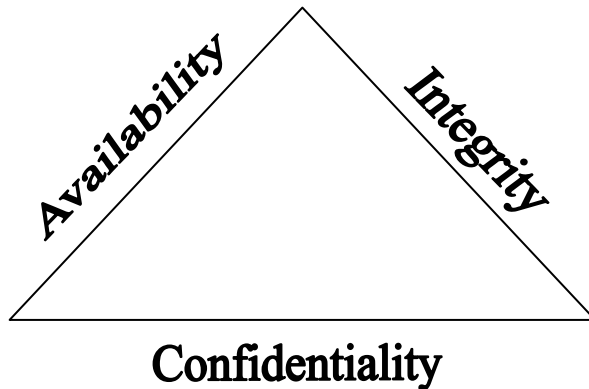
Figure 3.1 – CIA Triad
